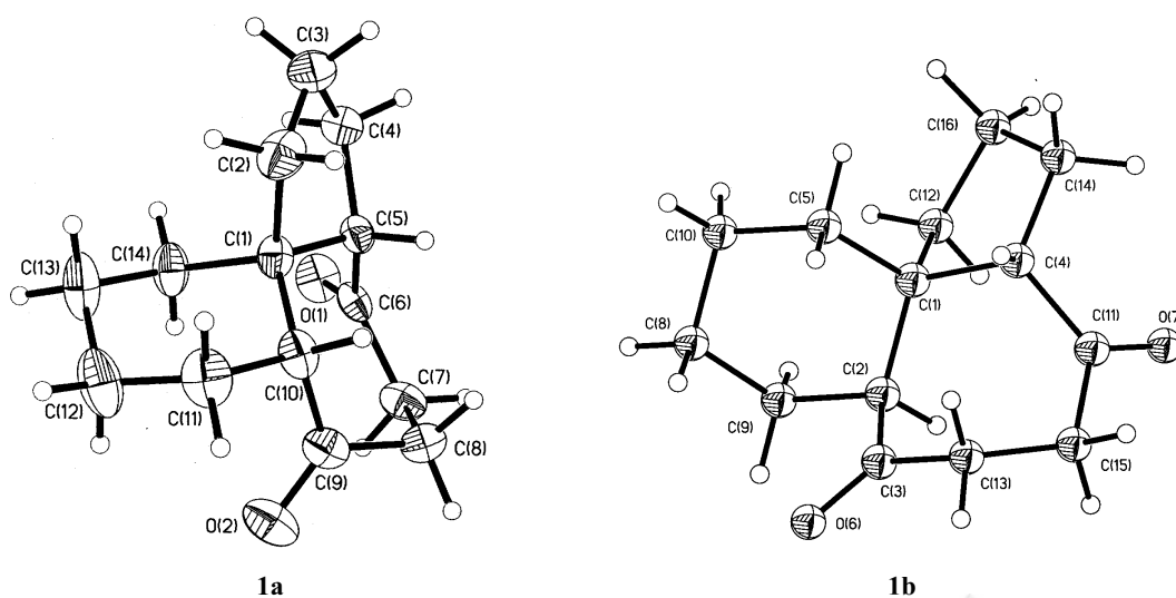
Fig. 1. ORTEP plots for X-ray crystal structures of 1a and 1b .
